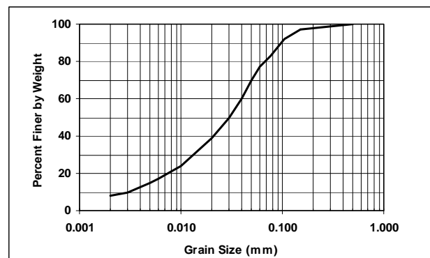
Figure 5. Grainsize curve of Kaministiquia River silt.
