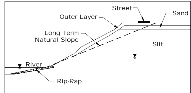
Figure 4. 2003 Kaministiquia River slope model.
