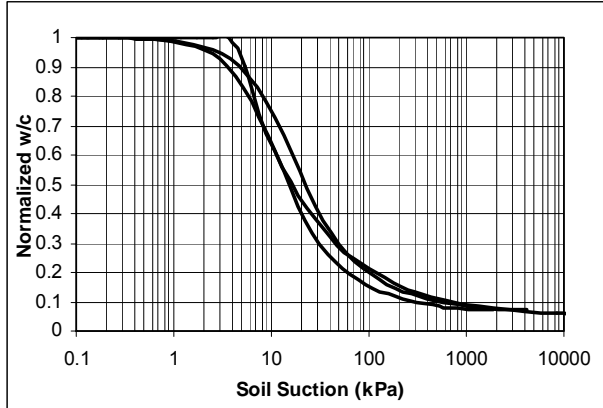
Figure 6. Estimated SWCC for Kaministiquia River silt.
